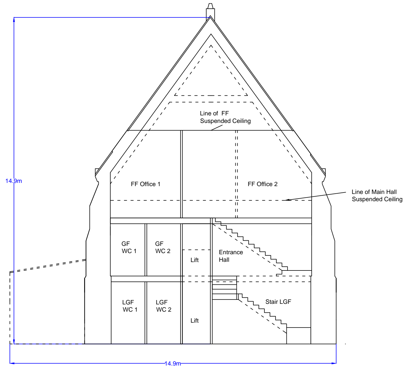
8DT17: 8 Derby Terrace North Section A, As Is Page 1 of 1, Scale 1:100 at A3
